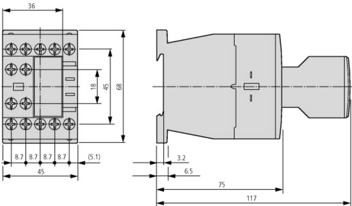
Contacteur with auxiliary contact module DILM32-XHI.../DILA-XHI...
